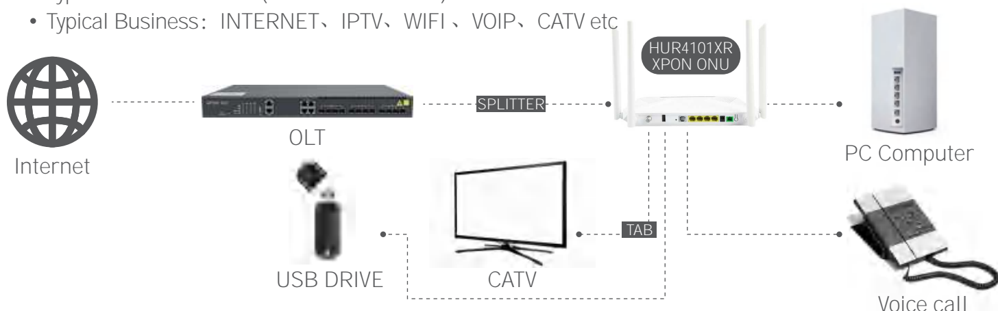
Figure: HUR4101XR Application Diagram
