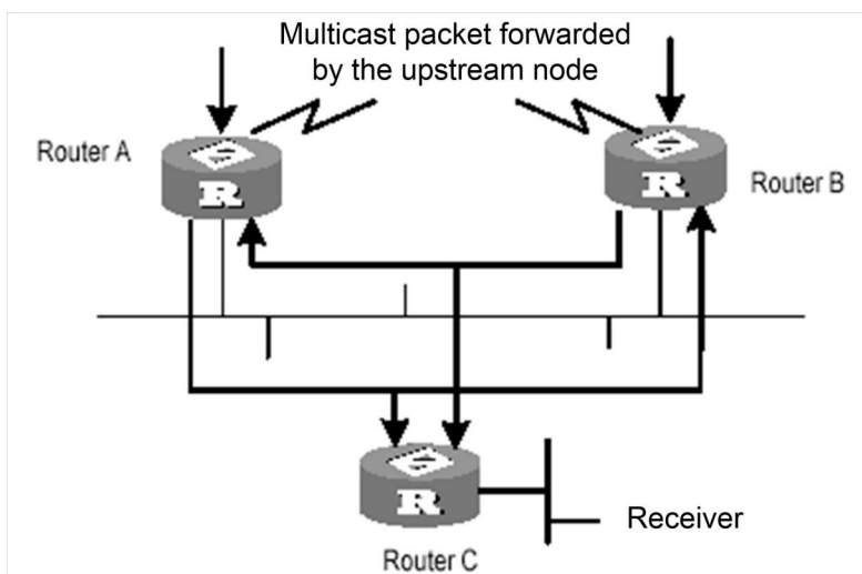
Assert mechanism
