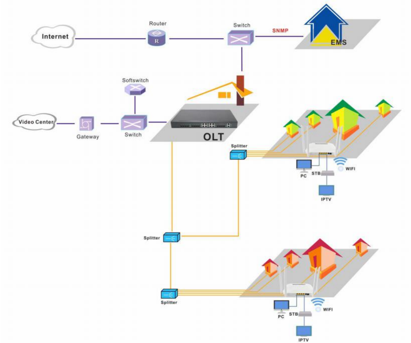
Figure: HUR4002XR Application Diagram
