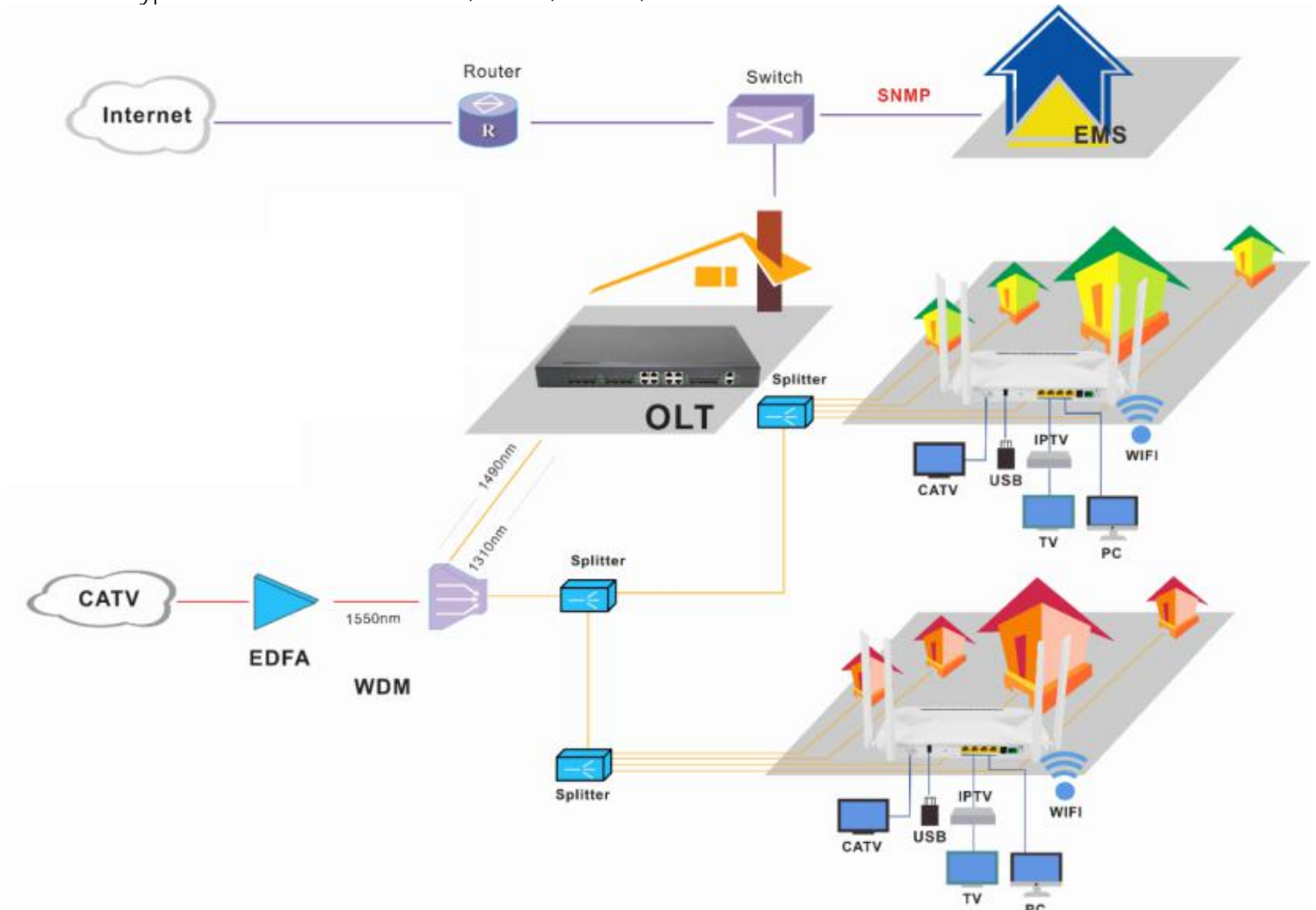
Figure: HUR4103XR Application Diagram
